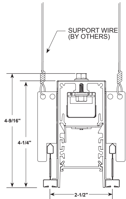
9/16 SCREW-SLOT
