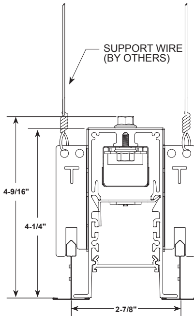
15/16 GRID
