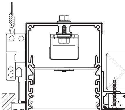
SCREW SLOT GRID + N1 (1/2" GYP) SCREW SLOT GRID + N5 (5/8" GYP)
