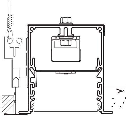
15/16" GRID + TILE
