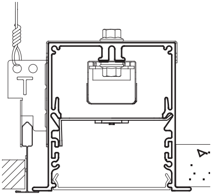
9/16" GRID + TILE
