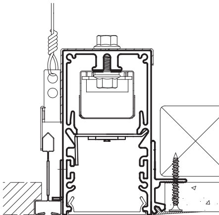
SCREW SLOT GRID + N1 (1/2" GYP) SCREW SLOT GRID + N5 (5/8" GYP)
