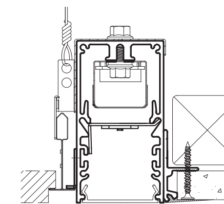
T 9/16" GRID + N1 (1/2" GYP) T 9/16" GRID + N5 (5/8" GYP)
