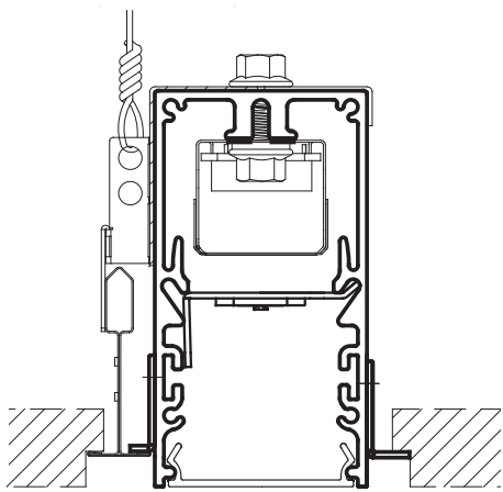
T 9/16" GRID + TEGULAR TILE
