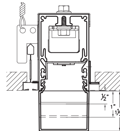
SCREW SLOT GRID TEGULAR TILE
