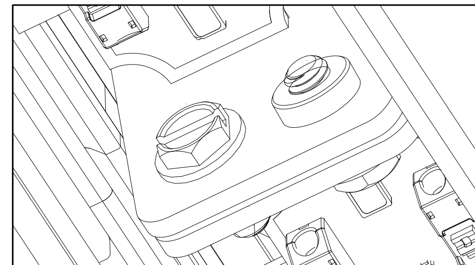
COMPLETE JOINT ASSEMBLY
