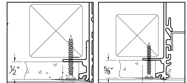
1/2" SHEETROCK
