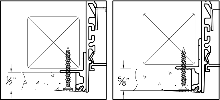
1/2" SHEETROCK 5/8" SHEETROCK CEILING OPTIONS
