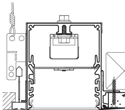
SCREW SLOT GRID + N1 (1/2" GYP) SCREW SLOT GRID + N5 (5/8" GYP)
