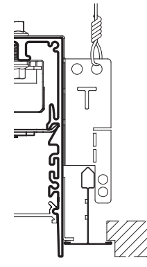
T15/16" GRID
