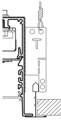
15/16" GRID
