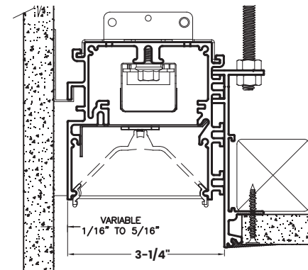
MLP3/N5 WITH 1" REGRESSED WALL GRAZER OPTIONAL
