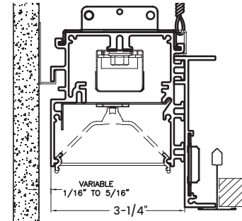
15/16" GRID WITH 1" REGRESSED WALL GRAZER OPTIONAL
