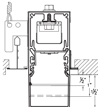
T15/16" GRID REGULAR TILE
