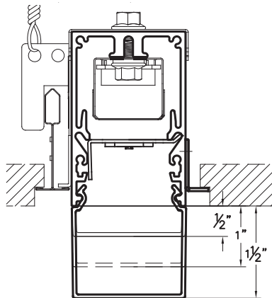
T9/16" GRID REGULAR TILE
