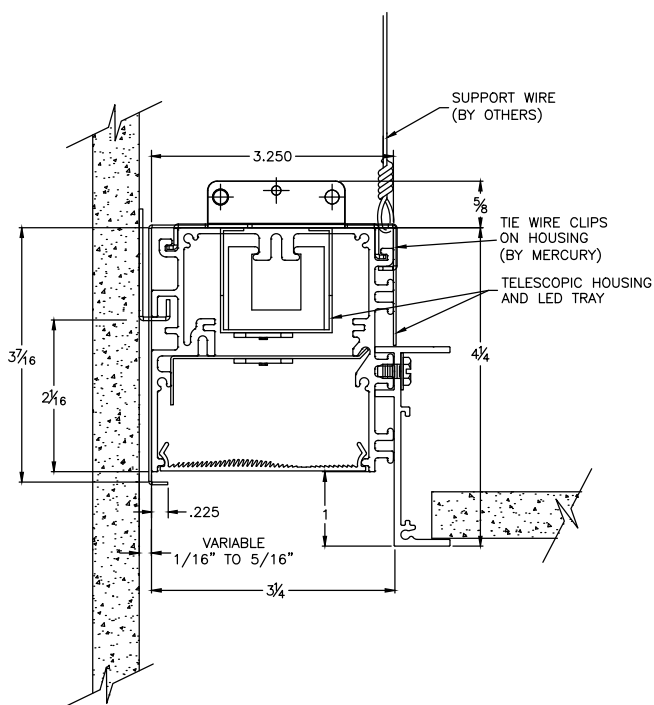
REGRESS TELE FLANGED ASYMMETRIC LENS
