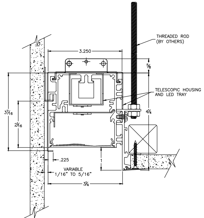
REGRESS TELE N5 ASYMMETRIC LENS
