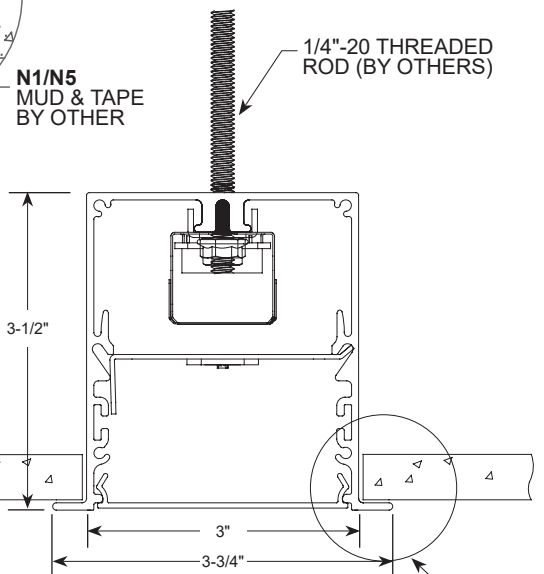
F OVERLAPPING TRIM
