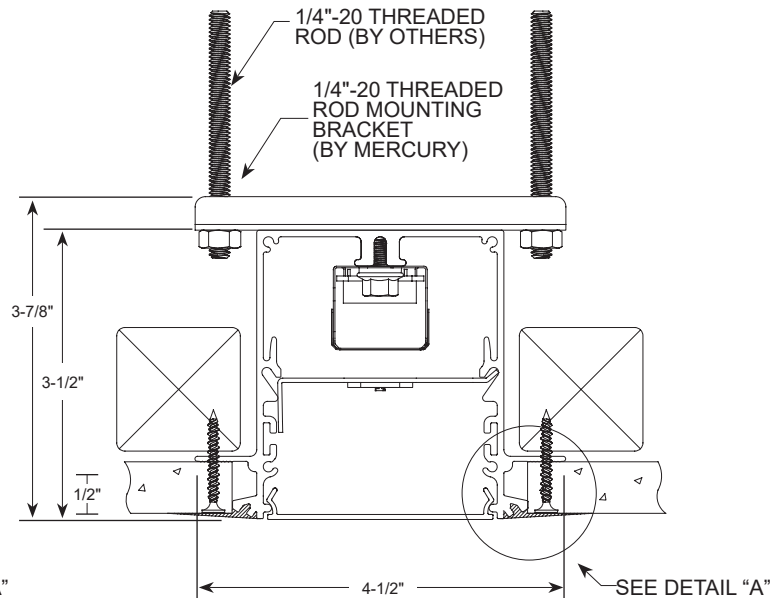
N5 TRIMLESS FIT FOR 5/8" DRYWALL (REQUIRES PLASTERING-IN AFTER INSTALLATION BY OTHERS)
