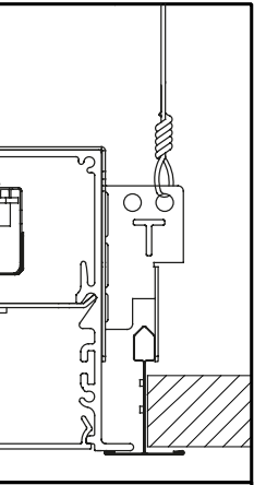
15/16 T-GRID
