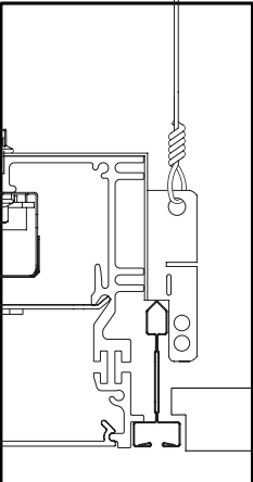
SCREW SLOT
