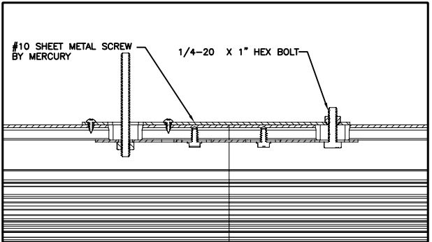
COMPLETE JOINT ASSEMBLY
