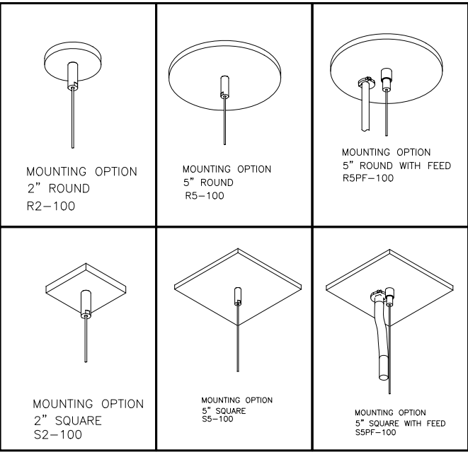
CANOPY OPTIONS
