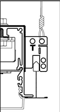
15/16 T-GRID
