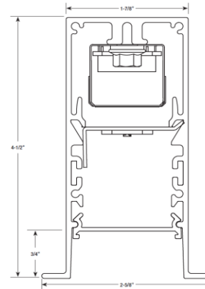
Luminaire Cross Section
