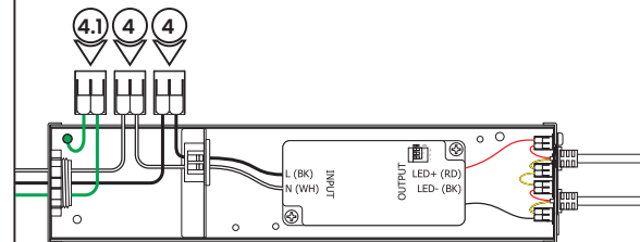
PRIMARY SIDE
