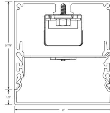
Luminaire Cross Section
